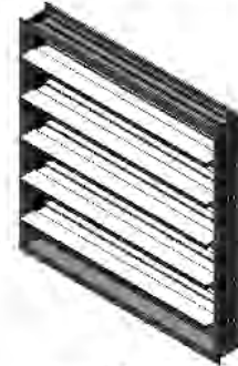
3965 Flanged-to-Duct
